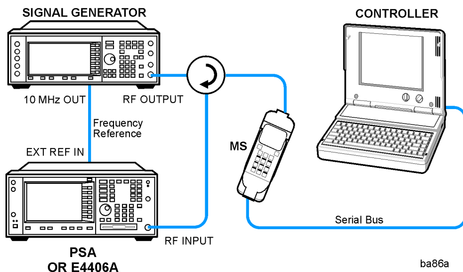
Figure 2-4 Adjacent Channel Power Ratio Measurement System
