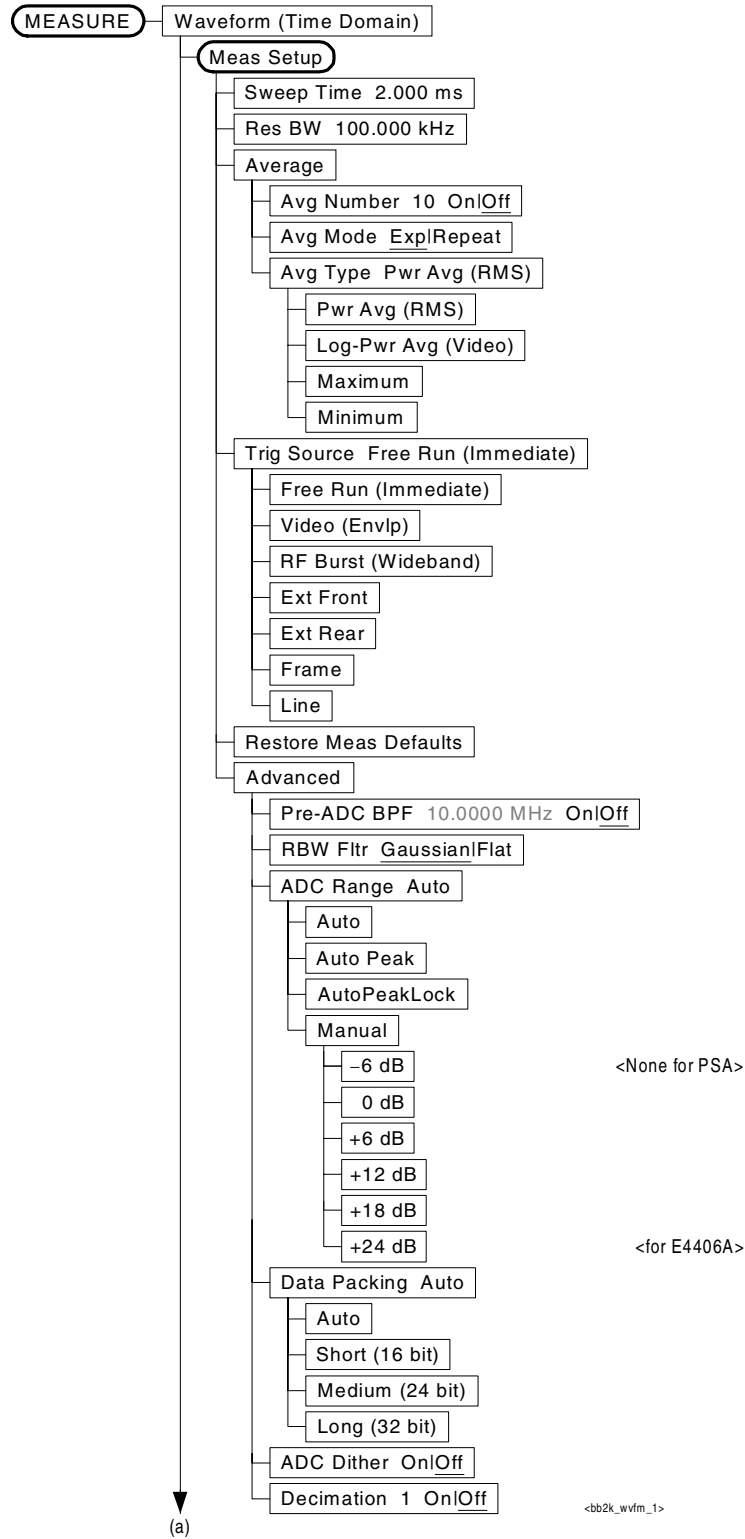
Figure 3-26 Waveform (Time Domain) Measurement Key Flow (1 of 3)
