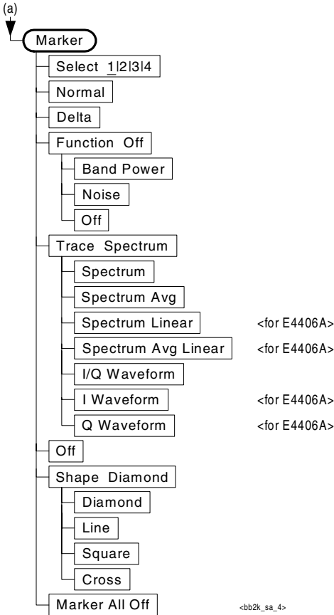
Figure 3-25 Spectrum (Freq Domain) Measurement Key Flow (4 of 4)
