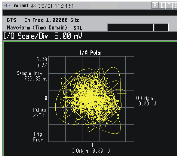
Figure 4-29 Waveform Measurement - I/Q Polar View
