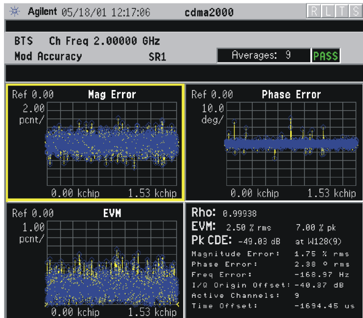
Figure 4-15 Modulation Accuracy Measurement - I/Q Error Quad View
