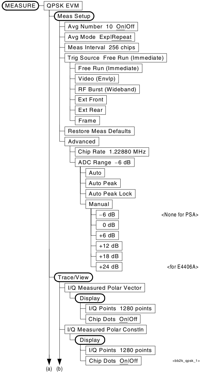
Figure 3-19 QPSK EVM Measurement Key Flow (1 of 2)
