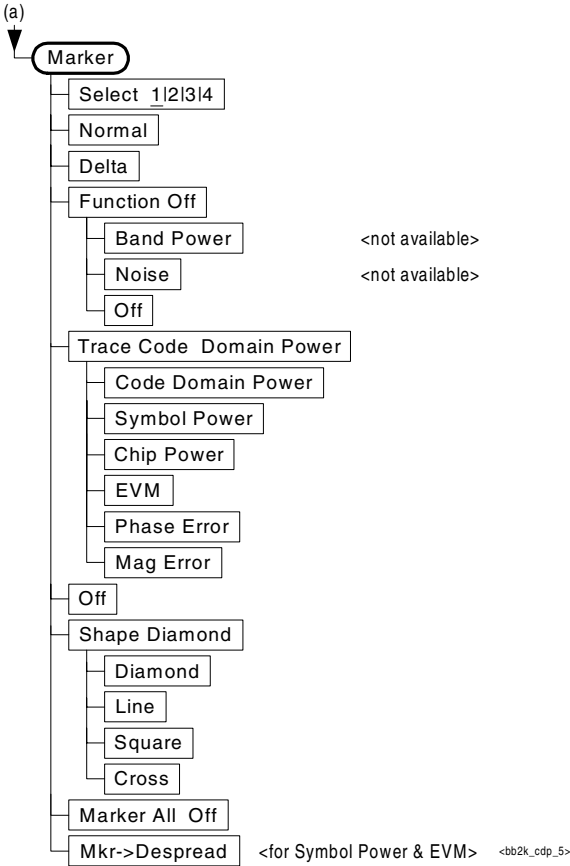
Figure 3-15 Code Domain Measurement Key Flow (5 of 5)
