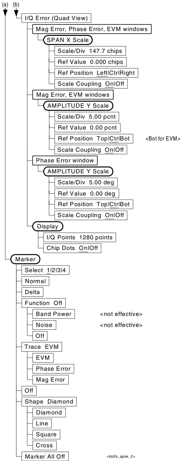
Figure 3-20 QPSK EVM Measurement Key Flow (2 of 2)
