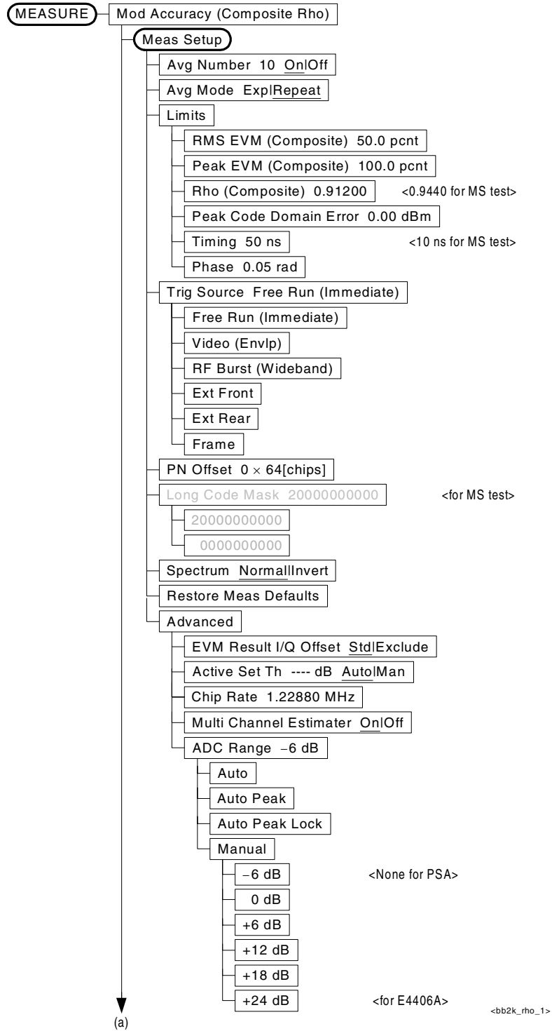
Figure 3-16 Modulation Accuracy Measurement Key Flow (1 of 3)
