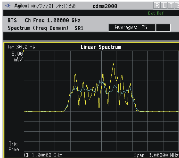
Figure 4-22 Spectrum Measurement - Linear Spectrum View (for E4406A)
