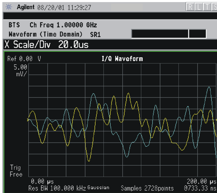
Figure 4-27 Waveform Measurement - I/Q Waveform View
