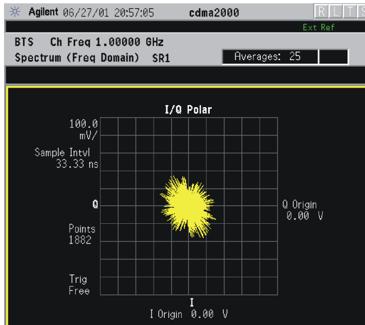
Figure 4-24 Spectrum Measurement - I/Q Polar View (for E4406A)
