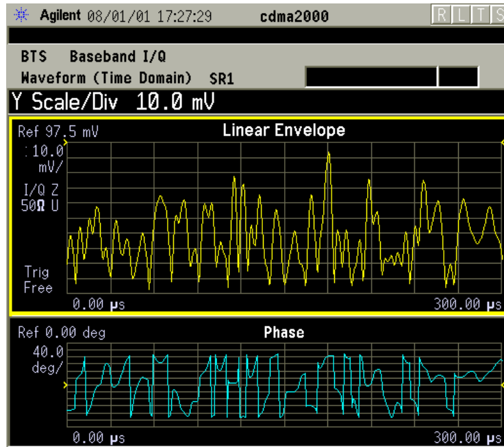
Figure 4-26 Waveform Measurement - Linear Envelope View
