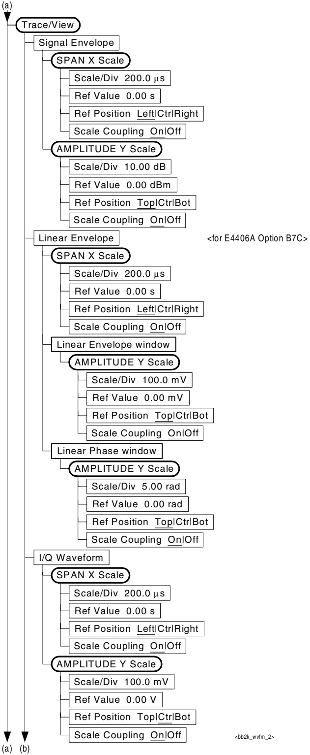
Figure 3-27 Waveform (Time Domain) Measurement Key Flow (2 of 3)
