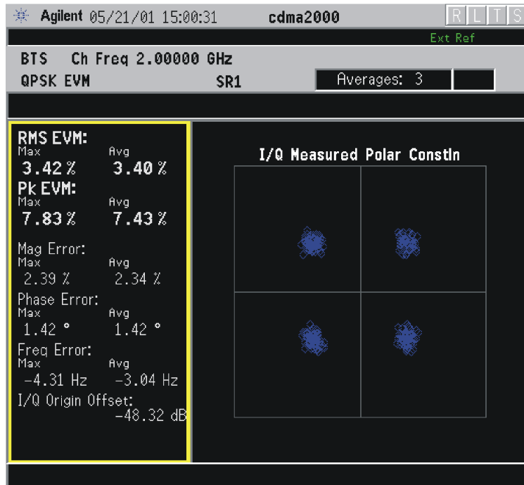
Figure 4-18 QPSK EVM Measurement - I/Q Polar Constellation View
