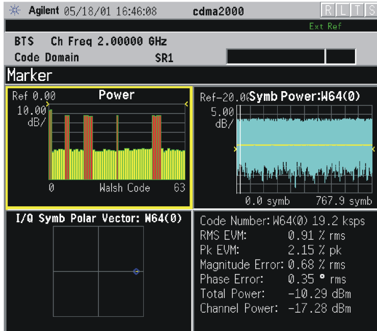
Figure 4-12 Code Domain Measurement - Code Domain with Quad View
