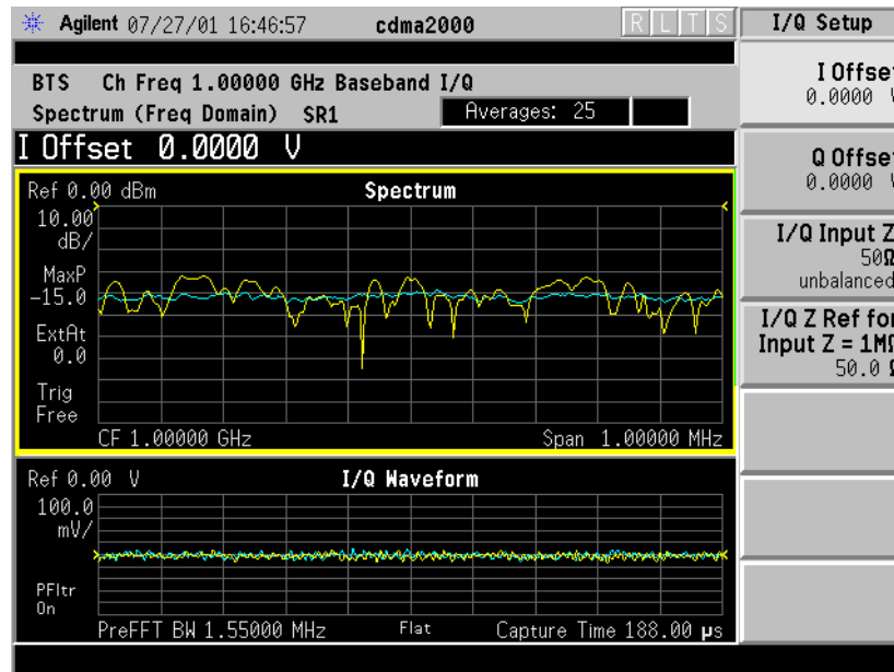
Figure 4-31 I/Q Setup Menu with Option B7C Baseband I/Q Inputs
