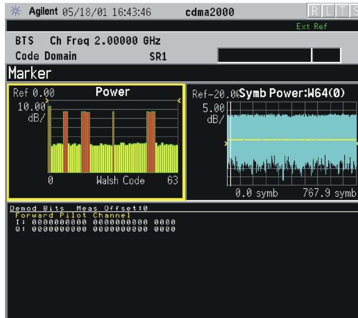
Figure 4-13 Code Domain Measurement - Demod Bits View
