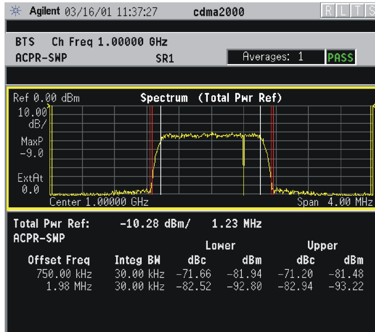
Figure 4-5 ACPR Measurement - Swept Spectrum (Total Pwr Ref) View
