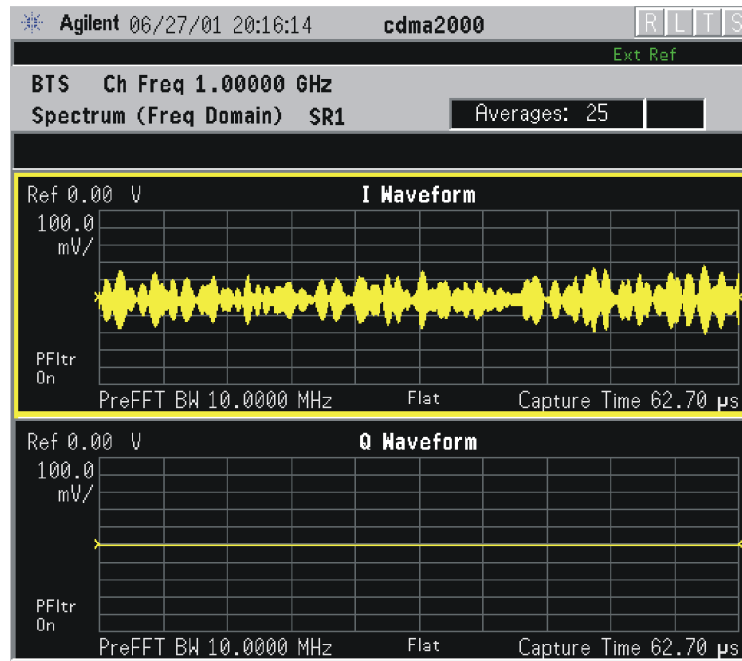
Figure 4-23 Spectrum Measurement - I and Q Waveform View (for E4406A)
