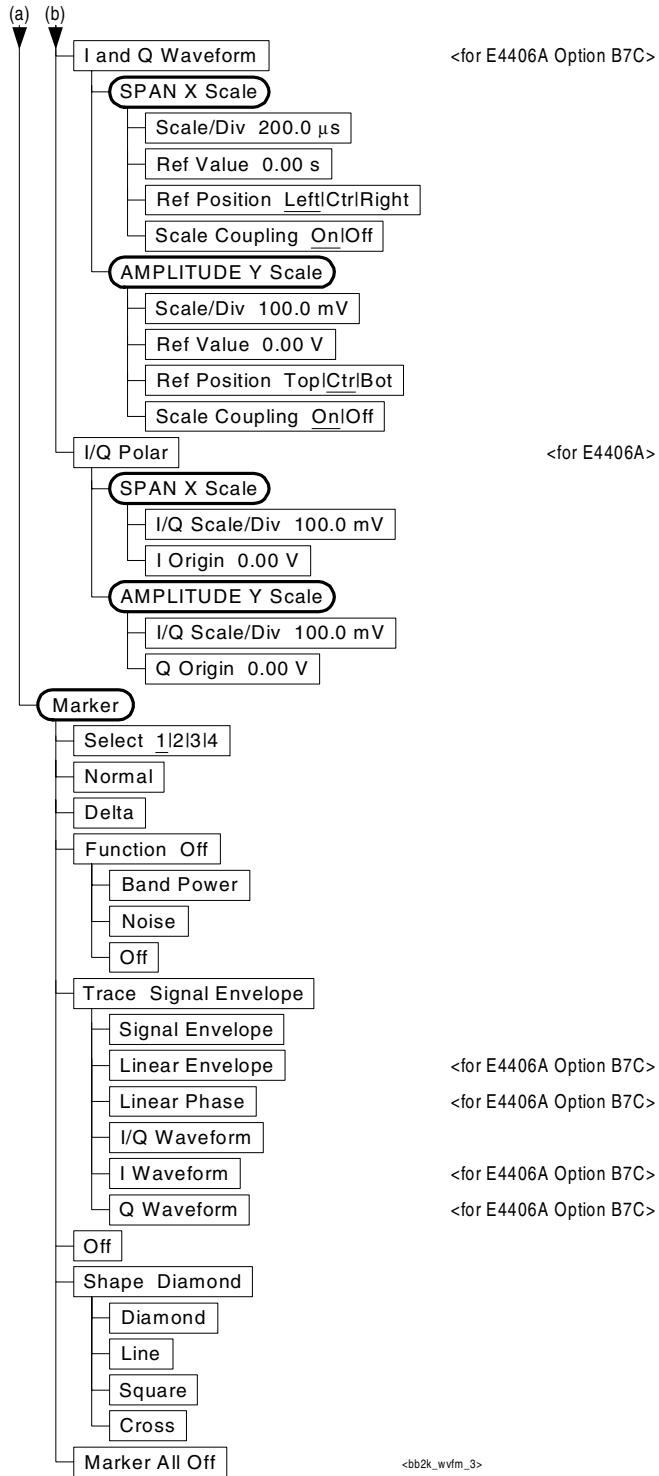
Figure 3-28 Waveform (Time Domain) Measurement Key Flow (3 of 3)
