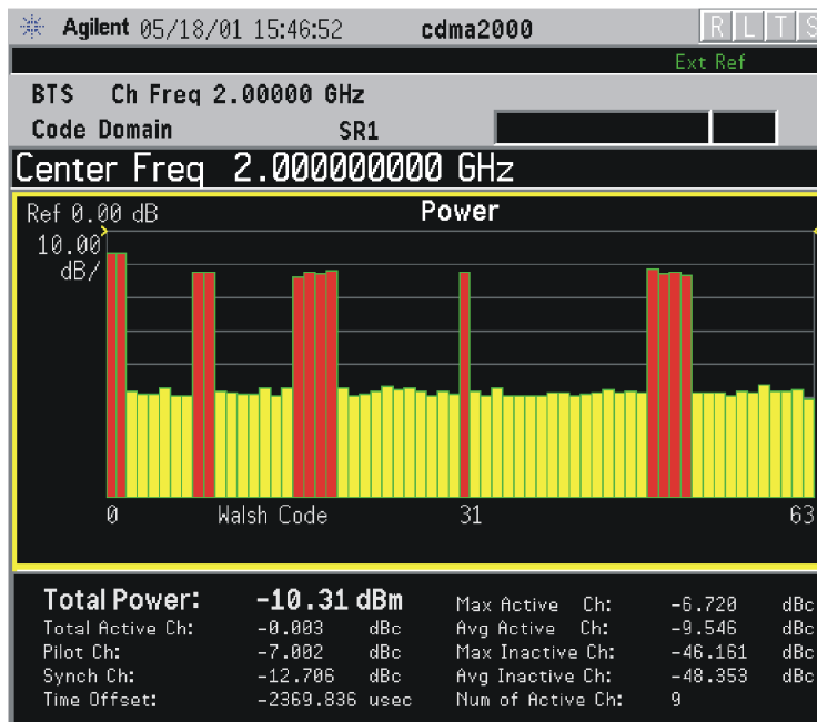
Code Domain Measurement - Power Graph View
