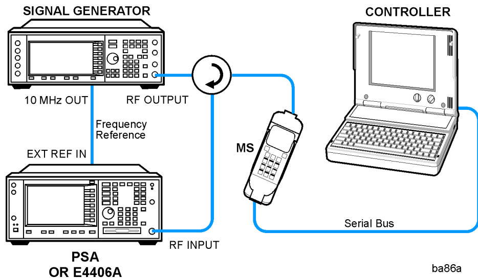
Figure 2-7 Occupied Bandwidth Measurement System
