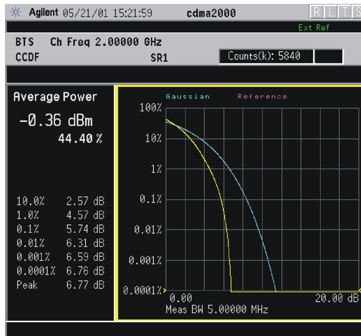
Figure 4-20 Power Statistics CCDF Measurement
