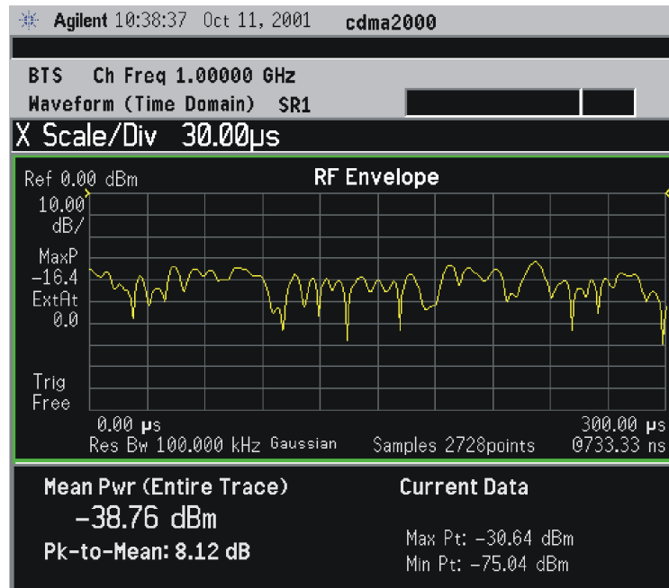
Waveform Measurement - RF Envelope View
