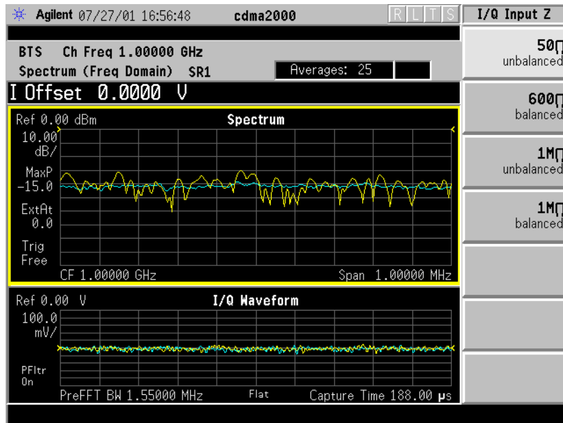
Figure 4-32 I/Q Input Z Menu - Option B7C Baseband I/Q Inputs
