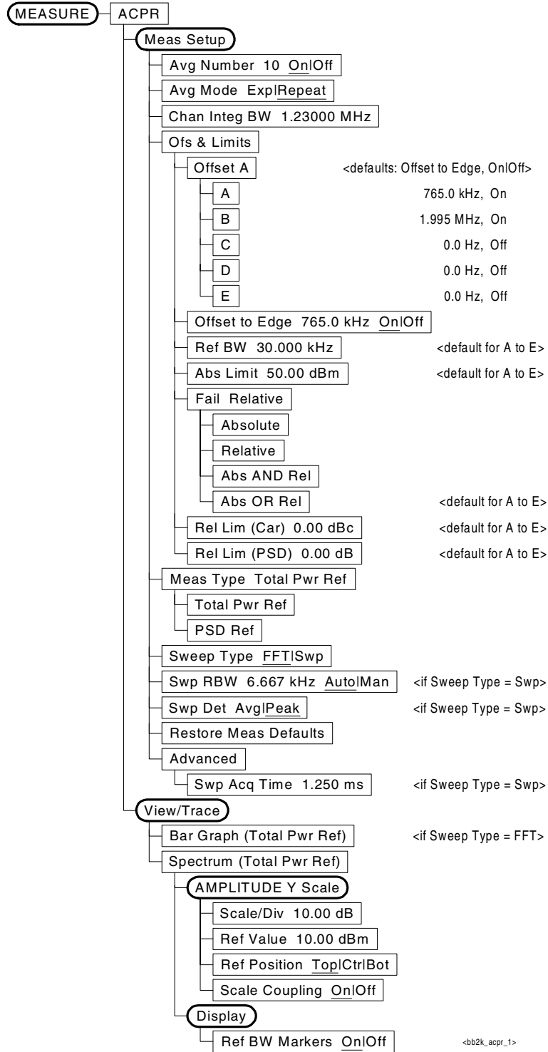
Figure 3-6 ACPR Measurement Key Flow
