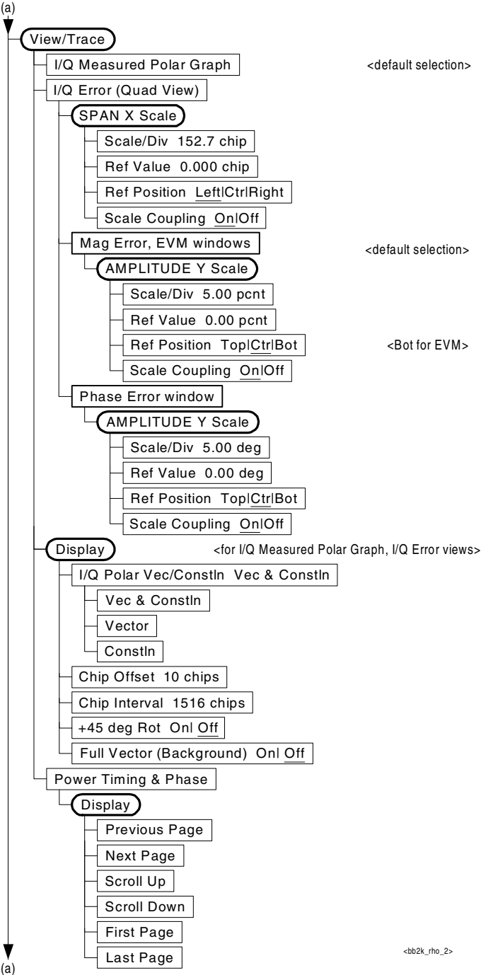
Figure 3-17 Modulation Accuracy Measurement Key Flow (2 of 3)
