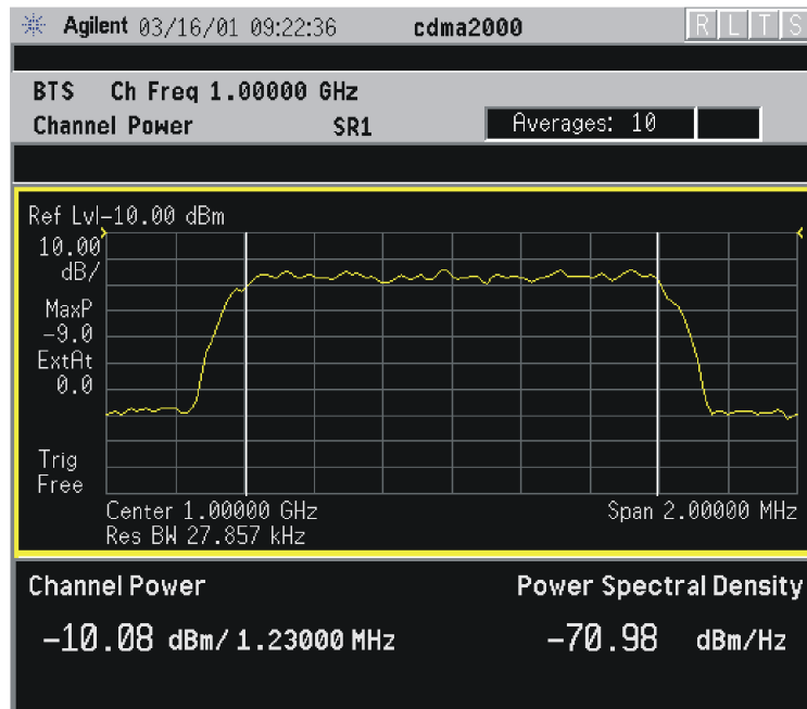
Channel Power Measurement
