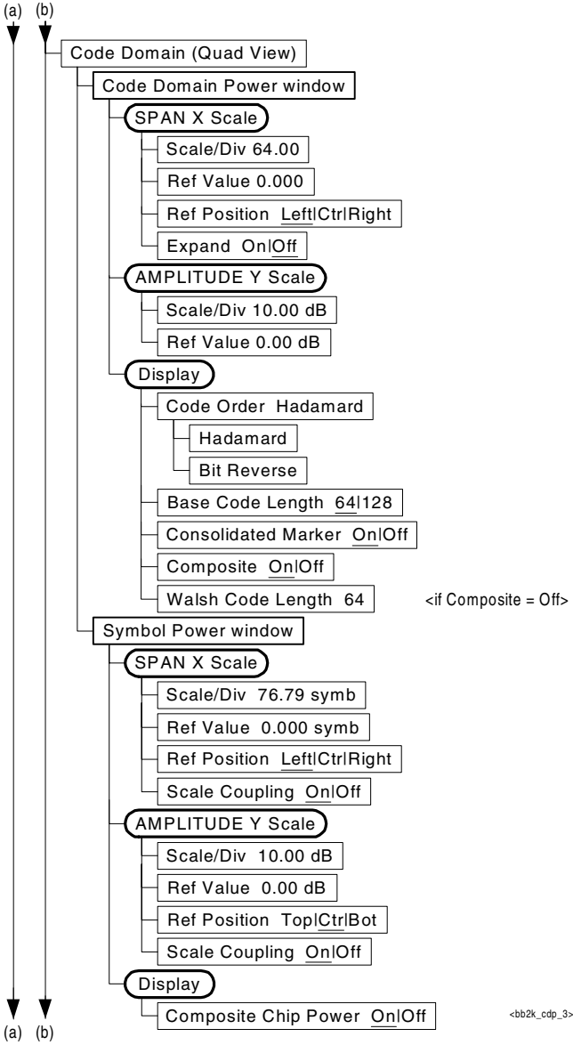
Figure 3-13 Code Domain Measurement Key Flow (3 of 5)
