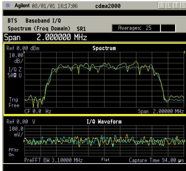
Figure 4-35 cdma2000 Spectrum View - Baseband I/Q Inputs
