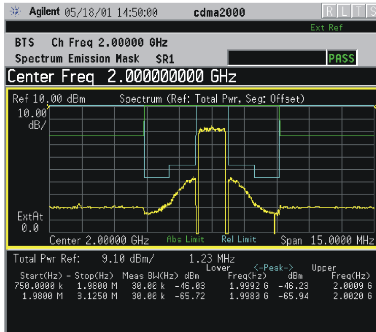
Figure 4-7 Spectrum Emission Mask Measurement - Offset Segment View
