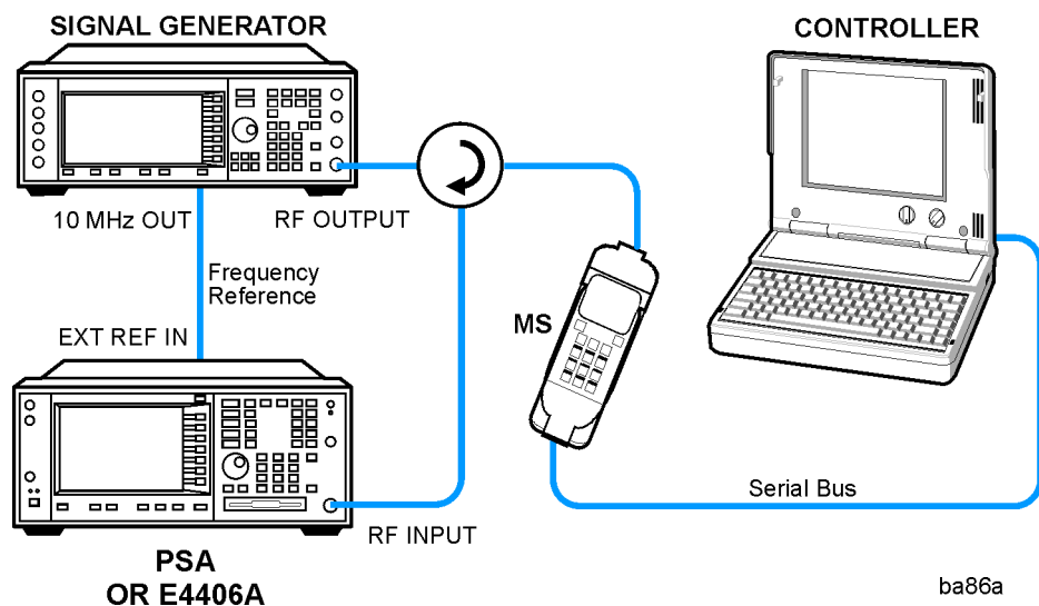
Figure 2-6 Spectrum Emission Mask Measurement System
