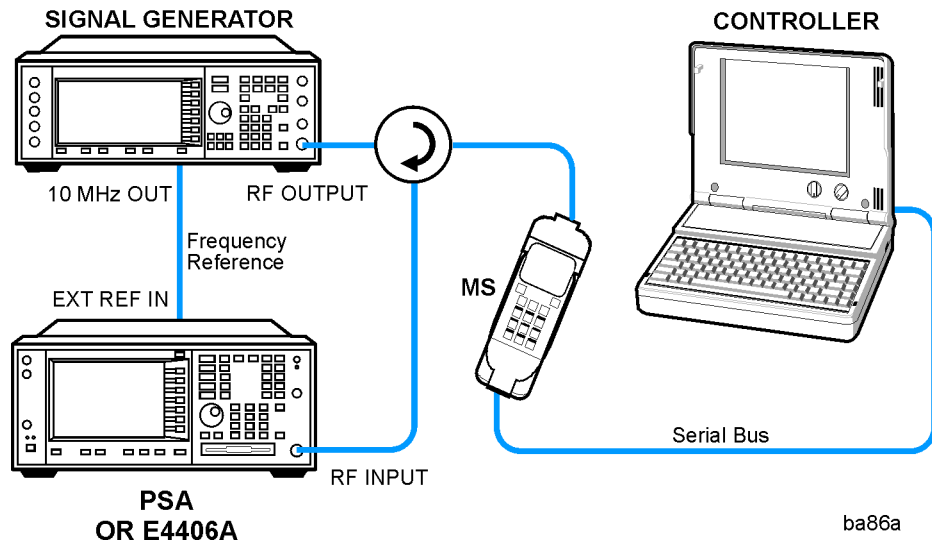
Figure 2-3 Channel Power Measurement System
