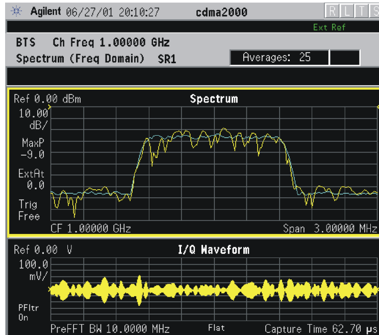
Spectrum Measurement - Spectrum and I/Q Waveform View
