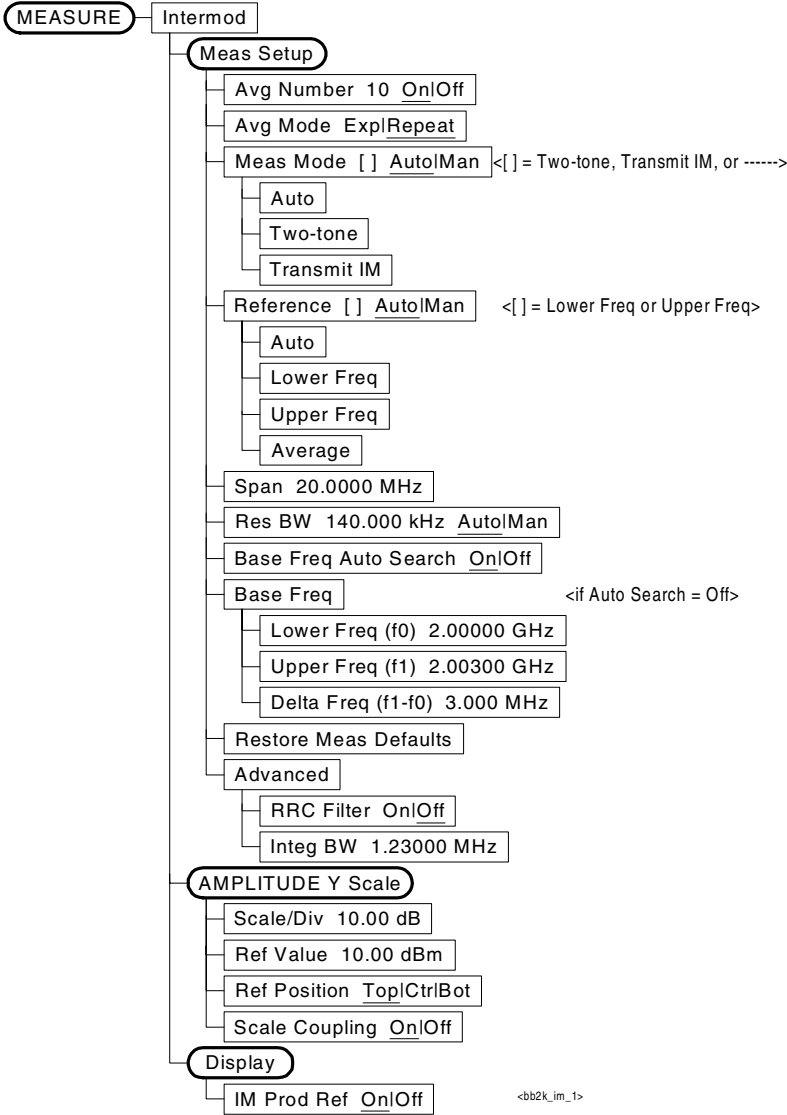
Figure 3-7 Intermodulation Measurement Key Flow
