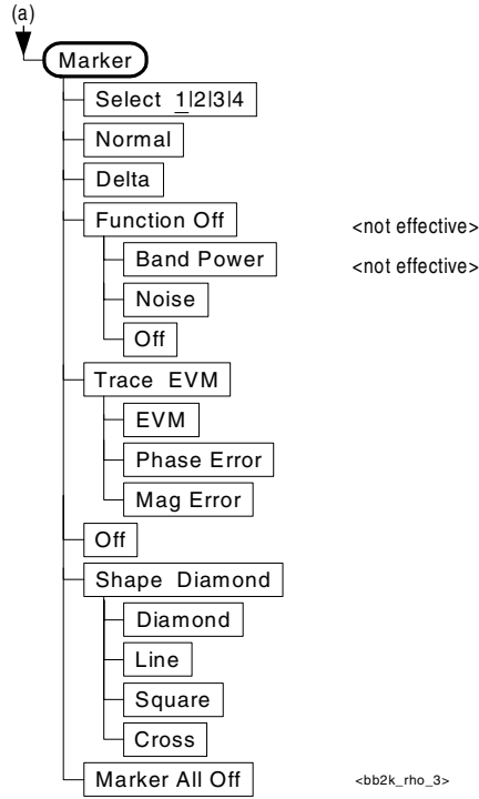
Figure 3-18 Modulation Accuracy Measurement Key Flow (3 of 3)
