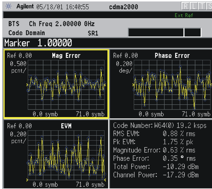
Figure 4-11 Code Domain Measurement - I/Q Error with Quad View
