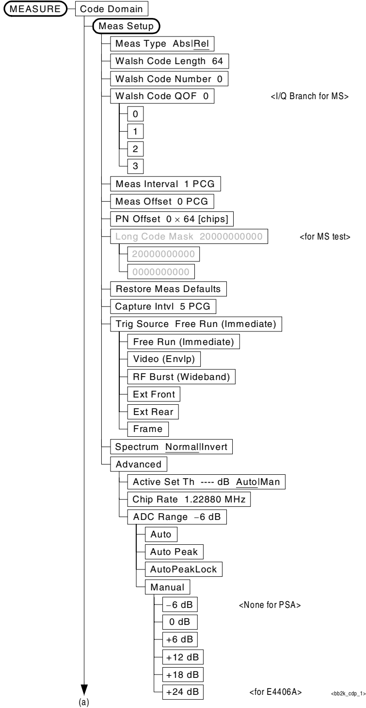
Figure 3-11 Code Domain Measurement Key Flow (1 of 5)
