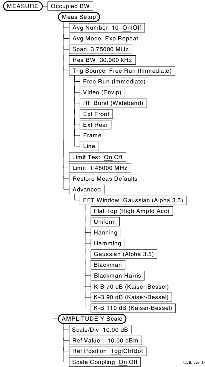
Figure 3-10 Occupied Bandwidth Measurement Key Flow
