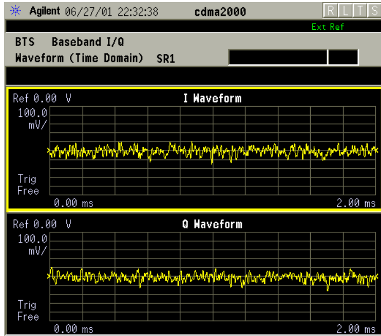
Figure 4-28 Waveform Measurement - I and Q Waveform View
