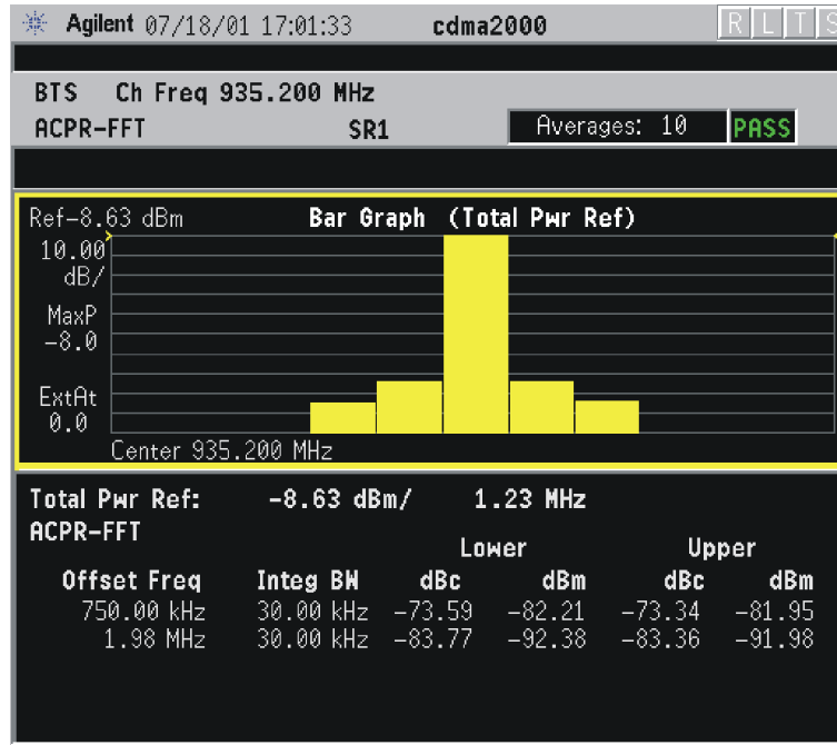
cdma2000 ACPR Measurement - FFT Bar Graph View
