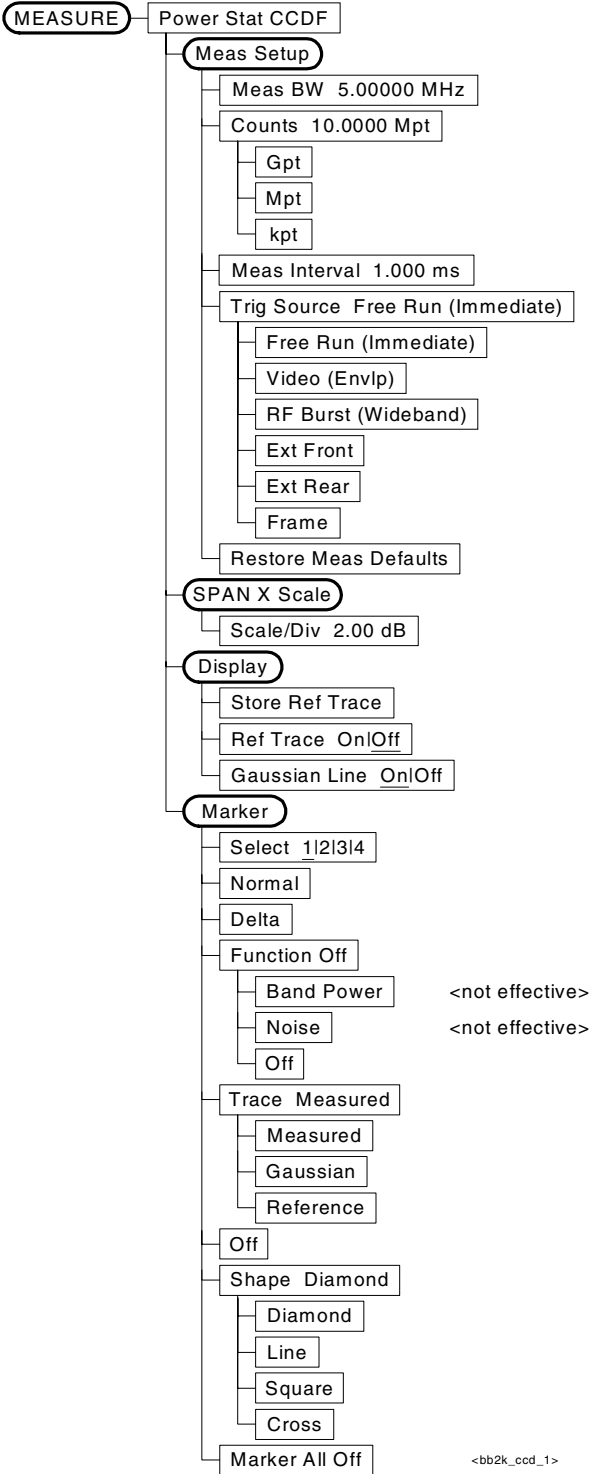
Figure 3-21 Power Statistics CCDF Measurement Key Flow
