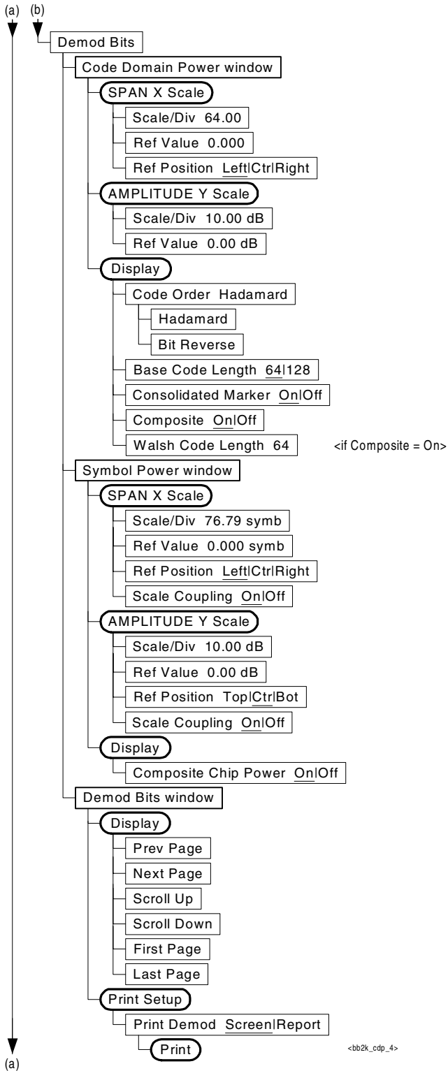
Figure 3-14 Code Domain Measurement Key Flow (4 of 5)
