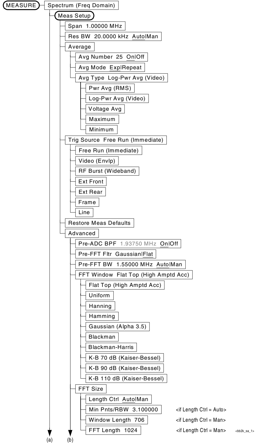
Figure 3-22 Spectrum (Freq Domain) Measurement Key Flow (1 of 4)
