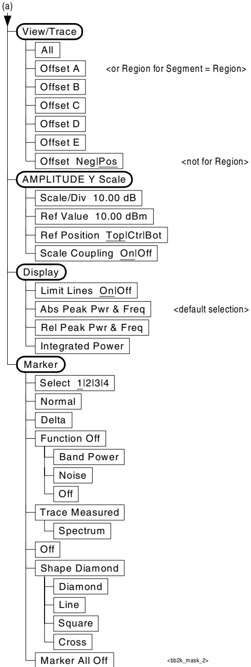
Figure 3-9 Spectrum Emission Mask Measurement Key Flow (2 of 2)
