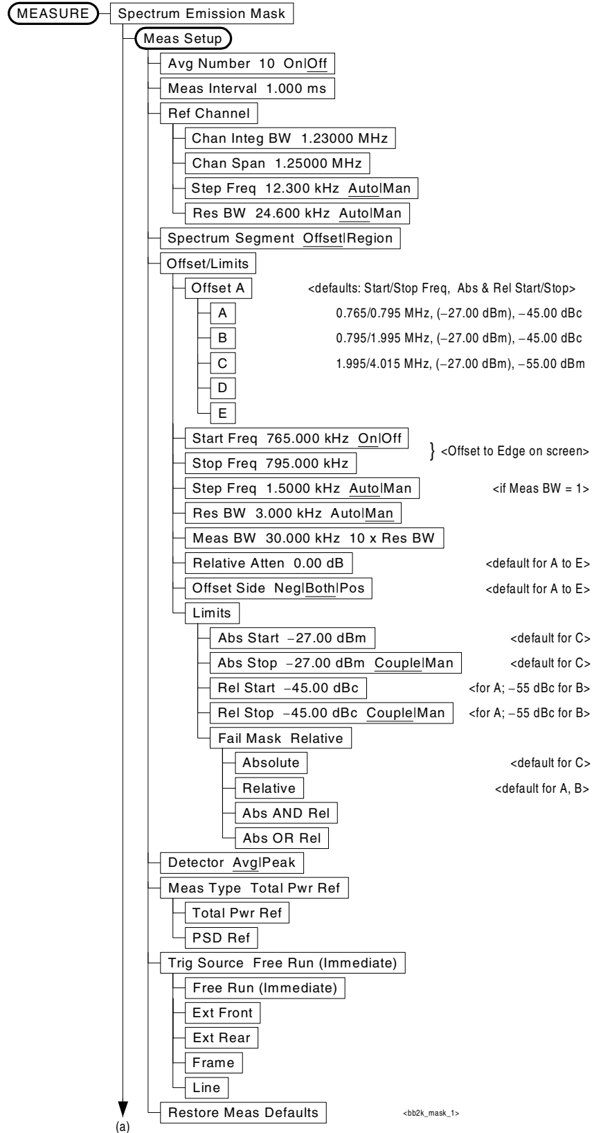
Figure 3-8 Spectrum Emission Mask Measurement Key Flow (1 of 2)
