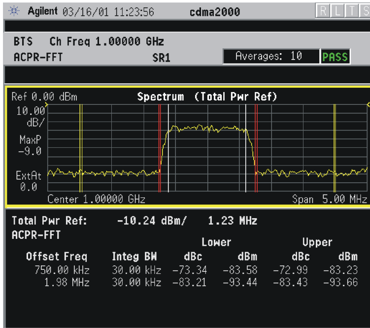
Figure 4-3 ACPR Measurement - FFT Spectrum (Total Pwr Ref) View
